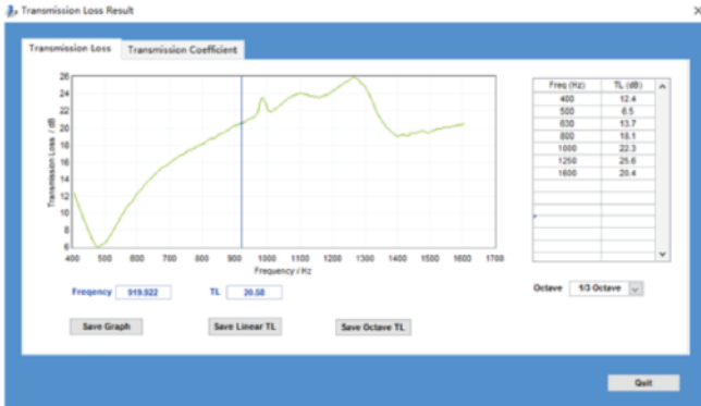
Sound insulation curve
